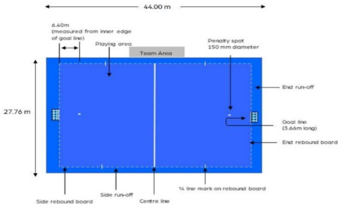
Figure 1 – Category 1 court layout
